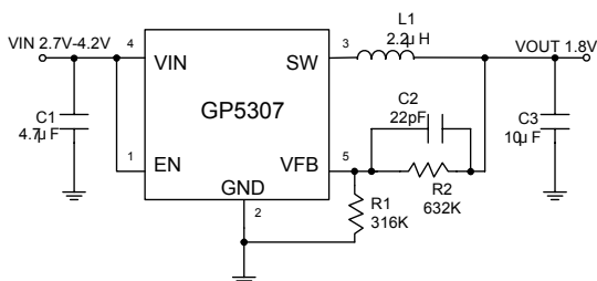
Figure 1. Basic Application Circuit with GP5307 adjustable version, V_{out} = 1.8V
