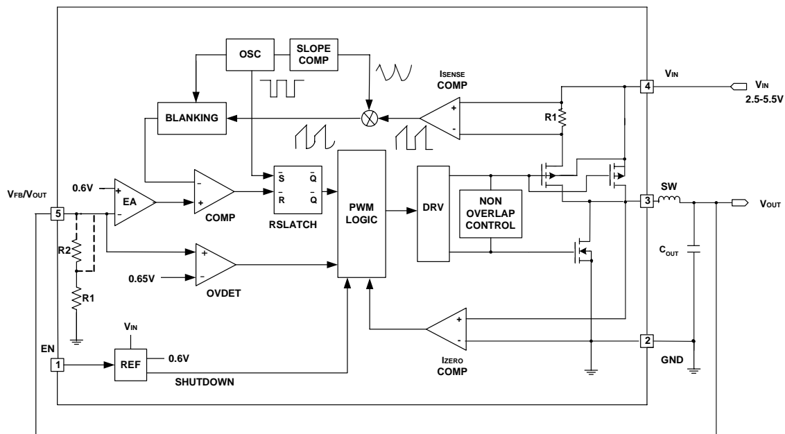
Figure 2. GP5307 Block Diagram
